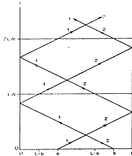
Fig. 1. Phase diagram for two particles.
