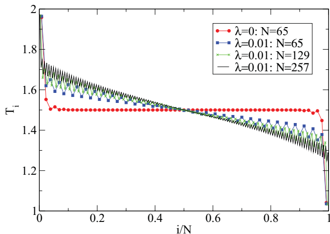
FIG. 5. (Color online) Temperature profiles with energy- and momentum-conserving noisy dynamics for a harmonic chain with an odd number of particles. Other parameters were taken to be m_a = 0.5 , m_b = 1.5 , \gamma_L = \gamma_R = 1.0 and T_L = 2.0, T_R = 1.0 .
