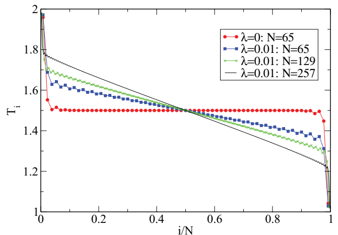
FIG. 7. (Color online) Temperature profiles with only energy-conserving noisy dynamics for a harmonic chain with an odd number of particles. Other parameters were taken to be m_a = 0.5 , m_b = 1.5 , \gamma_L = \gamma_R = 1.0 and T_L = 2.0, T_R = 1.0 .
