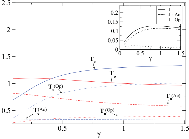
FIG. 2. (Color online) Temperatures at odd and even sites for a chain with even number of particles, plotted as a function of \gamma = \gamma_L = \gamma_R , m_a = 0.75, m_b = 0.25, k = 1, T_L = 1.5, T_R = 0.5 . We also plot separately the contributions of the acoustic and optical modes to the temperature at any site. The inset shows J and also the contributions of the acoustic and optical modes.
