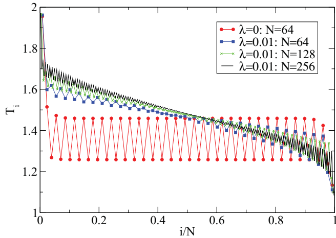
FIG. 4. (Color online) Temperature profiles with energy- and momentum-conserving noisy dynamics for a harmonic chain with even number of particles. Other parameters were taken to be m_a = 0.5 , m_b = 1.5 , \gamma_L = \gamma_R = 1.0 and T_L = 2.0, T_R = 1.0 .
