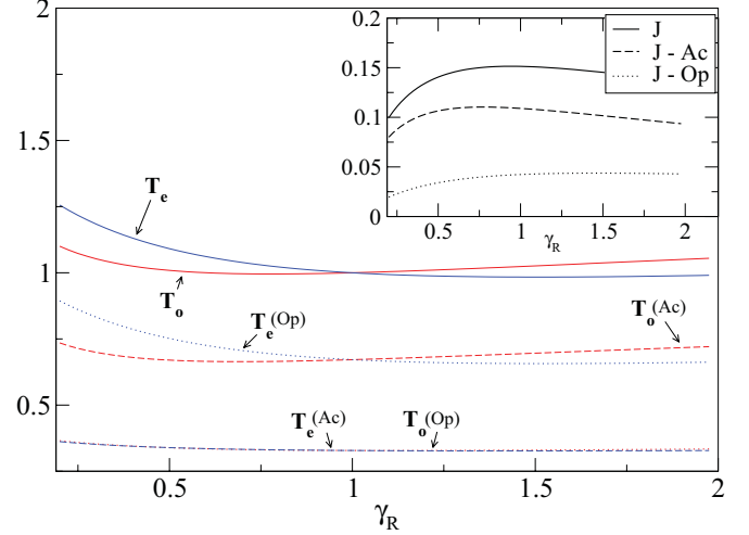
FIG. 3. (Color online) Temperatures at odd and even sites for a chain with odd number of particles, plotted as a function of \gamma_R with \gamma_L = 1 , m_a = 0.75, m_b = 0.25, k = 1, T_L = 1.5, T_R = 0.5 . We also plot separately the contributions of the acoustic and optical modes to the temperature at any site. The inset shows the variation of heat current with \gamma_R and also the contributions of the acoustic and optical modes.
