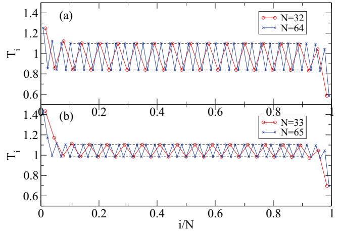
FIG. 1. (Color online) Temperature profiles for (a) system with even number of sites N = 32, 64 and with \gamma_L = \gamma_R = 1.0 and (b) system with odd number of sites N = 33, 65 and with \gamma_L = 1.5, \gamma_R = 0.5 . Other parameters were set to m_a = 0.75, m_b = 0.25, k = 1, T_L = 1.5, T_R = 0.5 . The mass of the first particle is always taken to be m_a . Note that in (a), the heavier particles are hotter, while in (b), the lighter particles are hotter. The horizontal dashed lines indicate the analytic predictions for N \rightarrow \infty , from Eqs. (11), (12).
