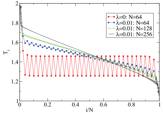
FIG. 6. (Color online) Temperature profiles with only energy-conserving noisy dynamics for a harmonic chain with even number of particles. Other parameters were taken to be m_a = 0.5 , m_b = 1.5 , \gamma_L = \gamma_R = 1.0 and T_L = 2.0, T_R = 1.0 .
