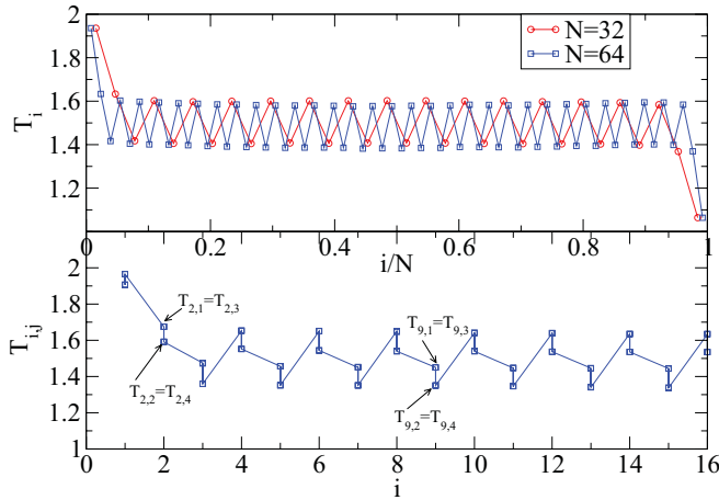
FIG. 8. (Color online) Simulation results for temperature profile for a two-dimensional N \times W strip of harmonically coupled particles with a periodic arrangement of masses. The sites on the strip are labeled (i, j) with i = 1, \dots, N and j = 1, \dots, W . Particles at sites with even i + j have mass m_a and others have masses m_b . Heat baths are attached to all sites on the layers i = 1 (temperature T_L ) and i = N (temperature T_R ). Periodic boundary conditions are imposed in the transverse ( j ) direction. Upper plot shows the average temperature on successive layers for chains of lengths N = 32 and N = 64 . There are oscillations in the transverse direction also and this is shown in the lower plot which shows the temperatures T_{i,j} on all sites of a section of the N = 64 chain. Note that from symmetry we have T_{i,j} = T_{i,j+2} , and this can be observed here. The width of the strips was taken to be W = 4 . The other parameters were taken to be m_a = 0.6 , m_b = 1.4 , \gamma_L = \gamma_R = 1.0 and T_L = 2.0, T_R = 1.0 .
