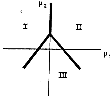
Fig. 2. 0 < T < J/k_B .
