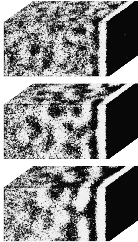
FIG. 4. Analogous to Fig. 1 but for a (very) strong-field case W_0/W_0^Y=4 , where the surface is completely wetted by the preferred component in equilibrium.
