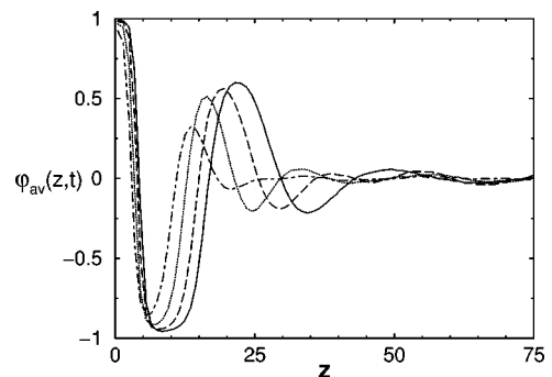
FIG. 5. Analogous to Fig. 2 but for the evolution depicted in Fig. 4 for the strong-field case. The profiles are shown at times t=50 (dot-dashed), 100 (dotted), 200 (dashed), and 275 (solid line).
