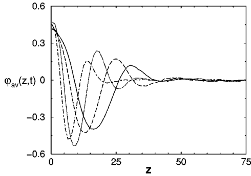
FIG. 2. Laterally averaged order parameter profiles \phi_{av}(z,t) as a function of z , the distance from the surface. Parameter values are the same as those for the evolution depicted in Fig. 1. The evolution times are t=50 (dot-dashed), 100 (dotted), 200 (dashed), and 275 (solid line).
