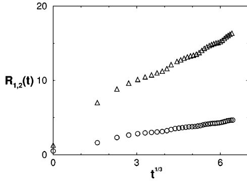
FIG. 6. Plot of first zero R_1(t) vs t^{1/3} (circles), and second zero R_2(t) vs t^{1/3} (triangles) of the laterally averaged profiles shown in Fig. 5.
