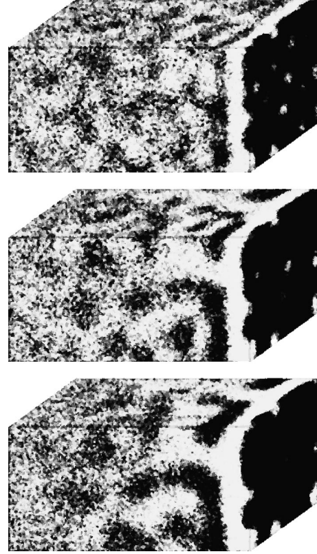
FIG. 1. Snapshots of the evolution after a critical quench for a weak-field case W_0/W_0^Y = 0.67 . The equilibrium surface morphology is partially wet. The times corresponding to the pictures are (from top to bottom) t = 60, 120, 180 .
